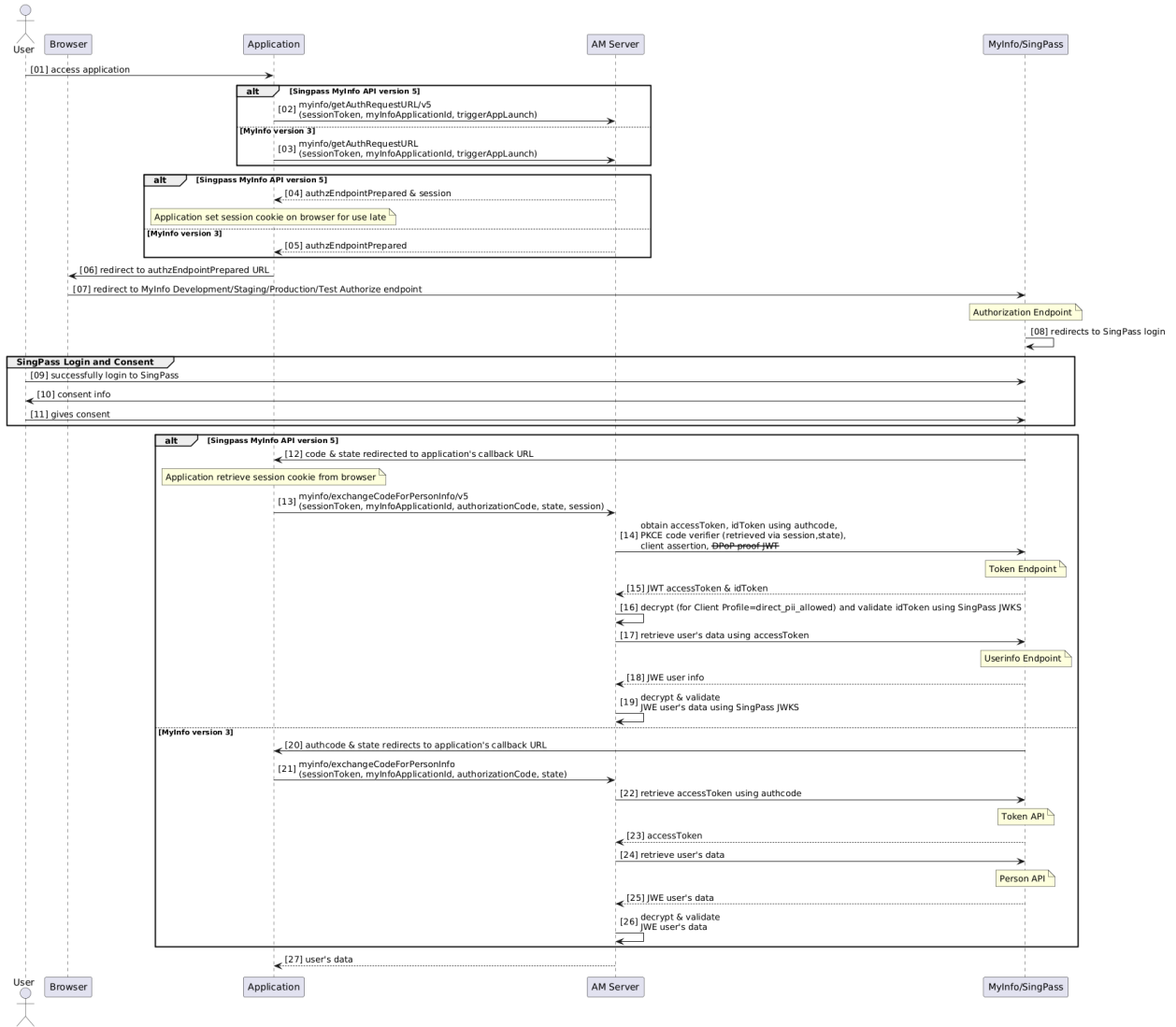
MyInfo Service Integration Sequence Diagram
